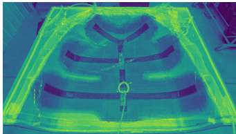
HSV V
