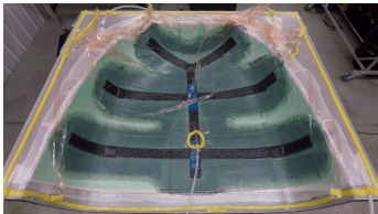
raw BGR
