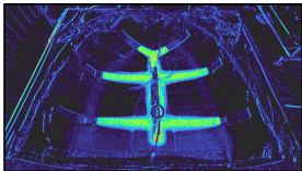
D_t, k_p = 0 (integrated)
