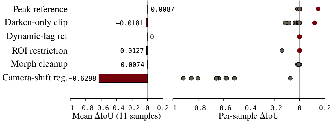
Fig. 17 Effect-size companion to Table Table 13. For each row in the table, the left bar is the eleven-sample mean \Delta\text{IoU} and the right strip is the eleven per-sample \Delta\text{IoU} values. Strips that cross zero identify primitives that are neutral or counterproductive on at least one sample, which is information the eleven-sample mean alone hides.
