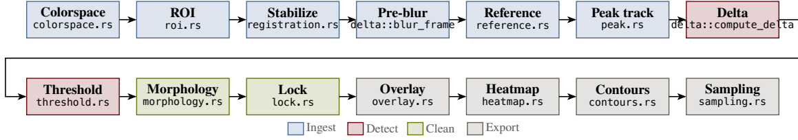
Fig. 1 Fourteen-stage integrated pipeline. Each frame flows from decode through an optional camera-shift registration and pre-delta blur, then through an appearance-difference comparison against a chosen reference, into a thresholded and morphologically cleaned mask, and finally through a temporal lock that stabilizes the boundary across frames. The same mask drives the binary, heatmap, and overlay renderers.
