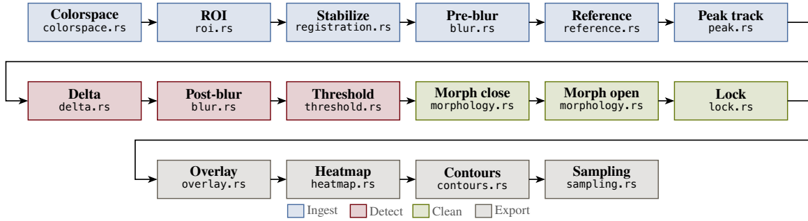
Fig. 4 Sixteen-stage integrated pipeline. Each frame flows from decode through an optional camera-shift registration and pre-delta blur, then through an appearance-difference comparison against a chosen reference, a post-delta blur, a threshold, paired morphological closing and opening passes, and finally a temporal lock that stabilizes the boundary across frames. The same mask drives the binary, heatmap, and overlay renderers.
