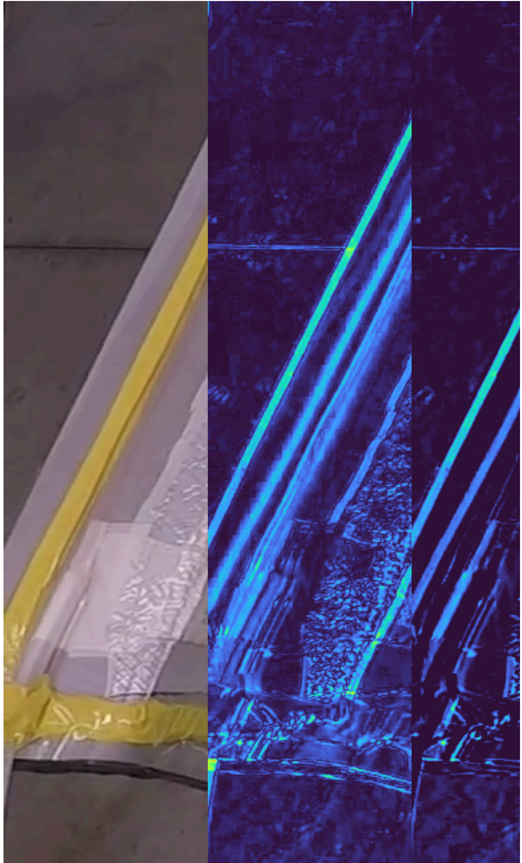
Fig. 3 Same input frame, two delta computations. The naive Euclidean delta (centre) lights up bright on the vacuum-bag specular highlight to the upper right of the laminate. The darken-only delta (right) discards the highlight and isolates the front. The early-fill front in the lower part of the panel is visible in both, though more cleanly in darken-only.
