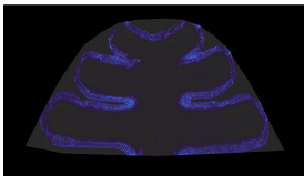
running EMA
