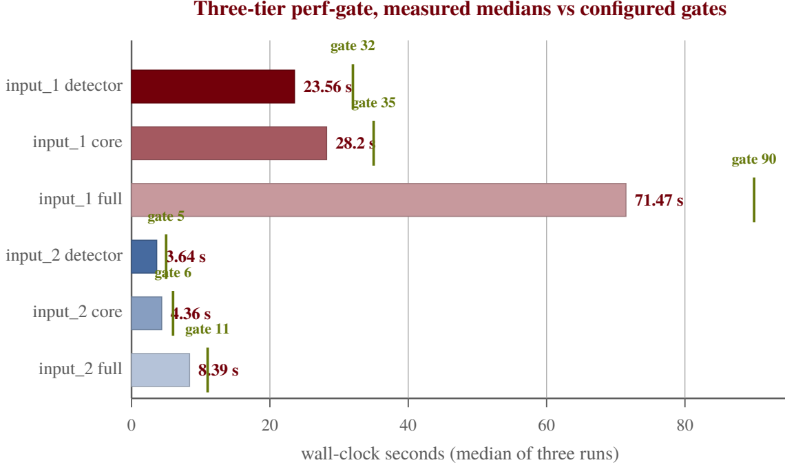
Fig. 9 Wall-clock medians for the integrated configuration on the high-resolution input_1 and time-lapse input_2 clips, broken down into the algorithm cost (detector tier), the algorithm plus MP4 encode (core tier), and the algorithm plus MP4 encode plus per-frame Portable Network Graphics (PNG) and Common Objects in Context (COCO) export (full tier). Hash marks indicate the pass/fail budgets enforced by the regression harness. The detector tier corresponds to roughly 30 frames per second on input_1 . Three-implementation aggregate wall-clock against the Python reference and the CUDA implementation is reported in Table Fig. 10 once the CUDA close-out completes.
