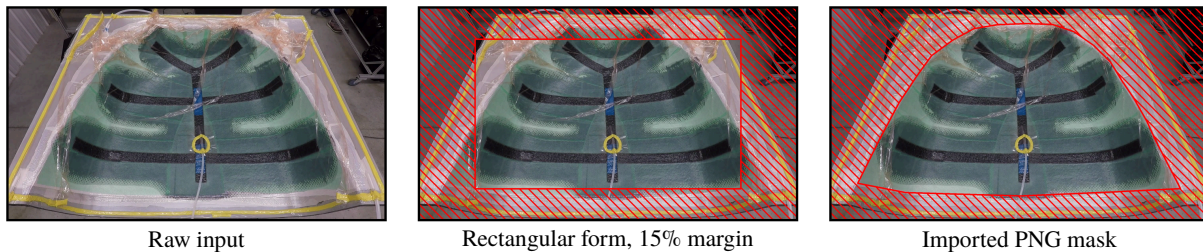
Fig. 4 Three forms of the ROI mask R on the canonical input frame, with pixels outside the ROI marked by red diagonals.
