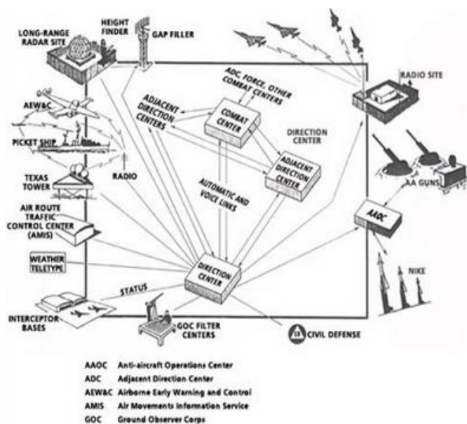
Figure 1 – a graphical representation of the SAGE air defense system's high level design schema
