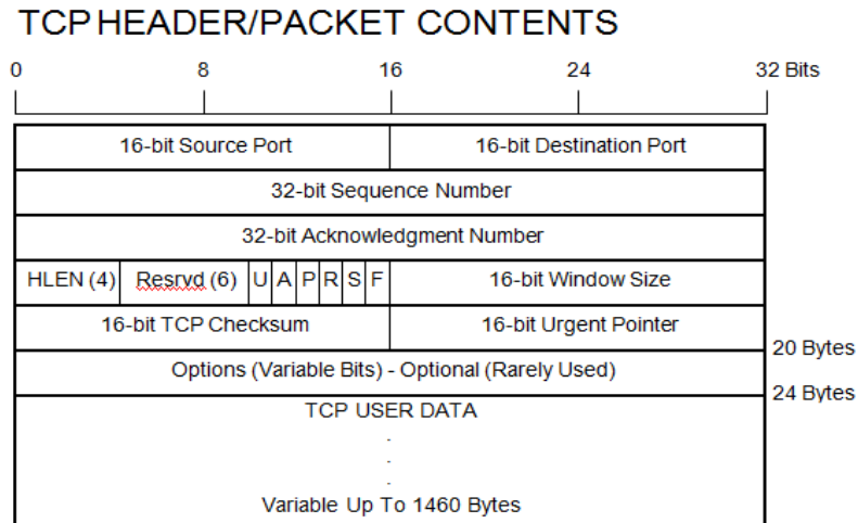
Figure 4 – TCP/IP Header
