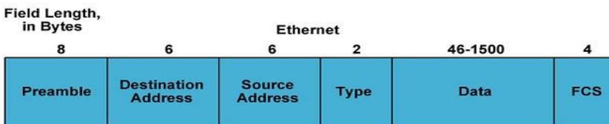
Figure 6 – Byte sizes and partitioning of a typical Ethernet frame shown
