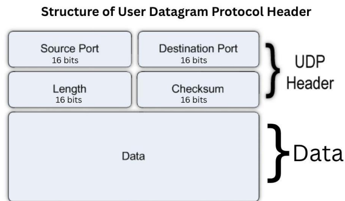
Figure 5 – UDP Header
