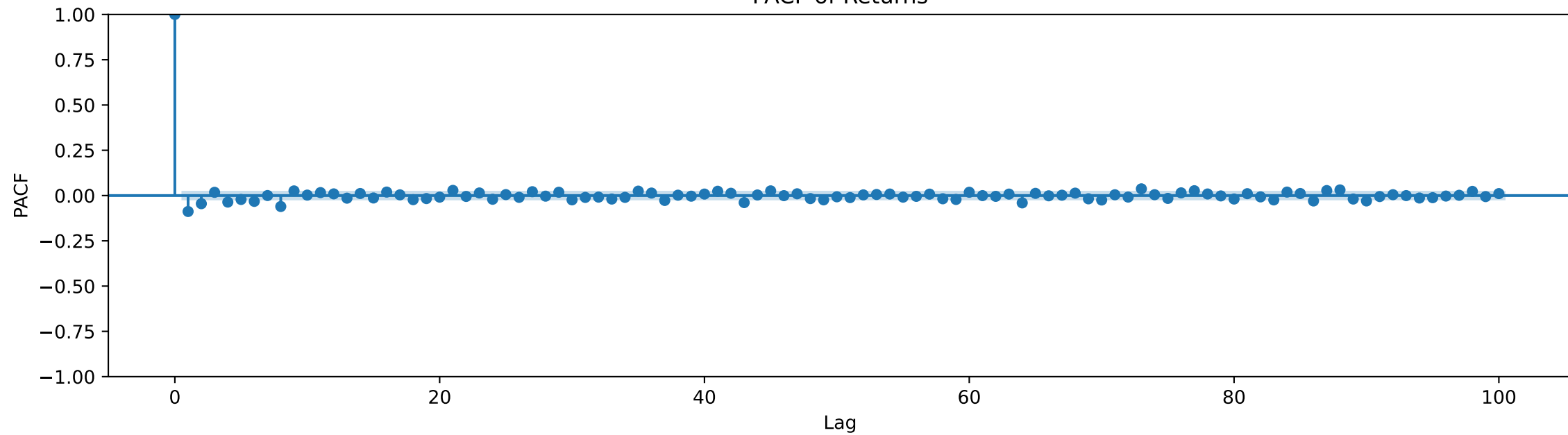
PACF of Returns
