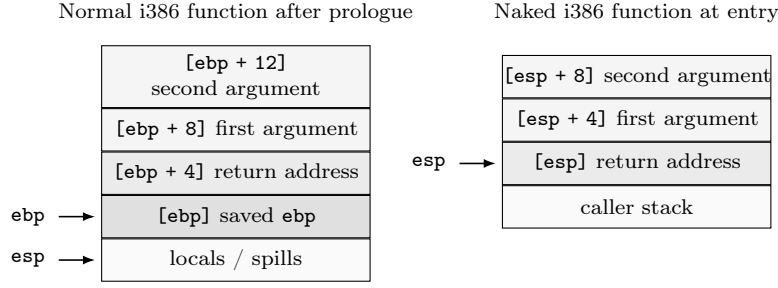
Рис. 2: i386 stack view for ordinary and naked CPL functions. In this target, ordinary functions use 32-bit registers such as eax , ebx , ecx , edx , esp , and ebp ; without push ebp ; mov ebp, esp , the backend addresses arguments from esp rather than from ebp .
