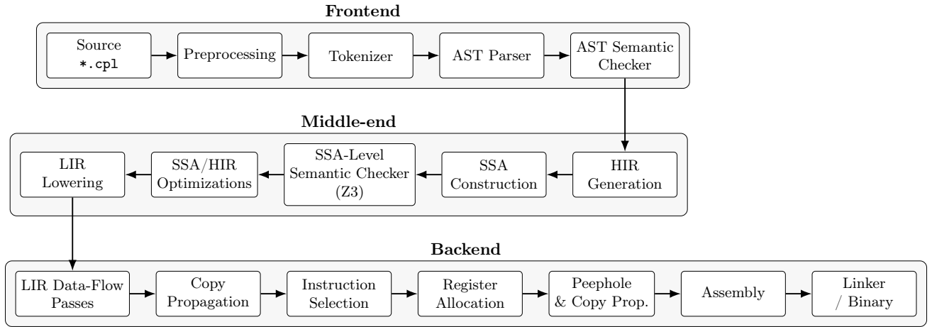
Рис. 1: Graphical overview of the CPL compiler architecture. The pipeline is arranged in three phases to preserve readability in a two-column layout while retaining the execution order.
