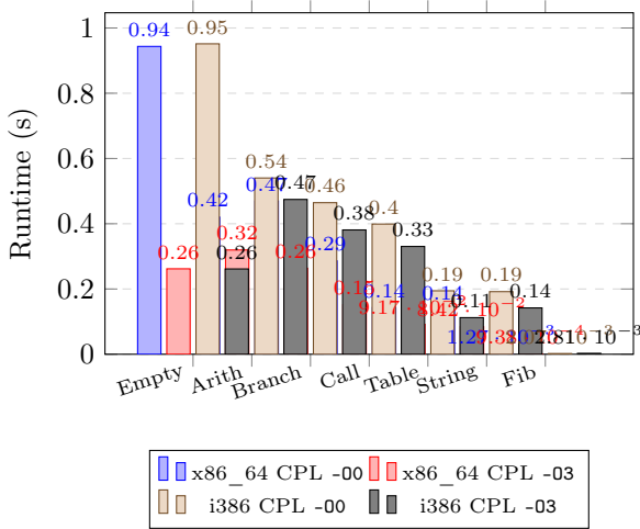
Рис. 4: Optimization effect within CPL.
