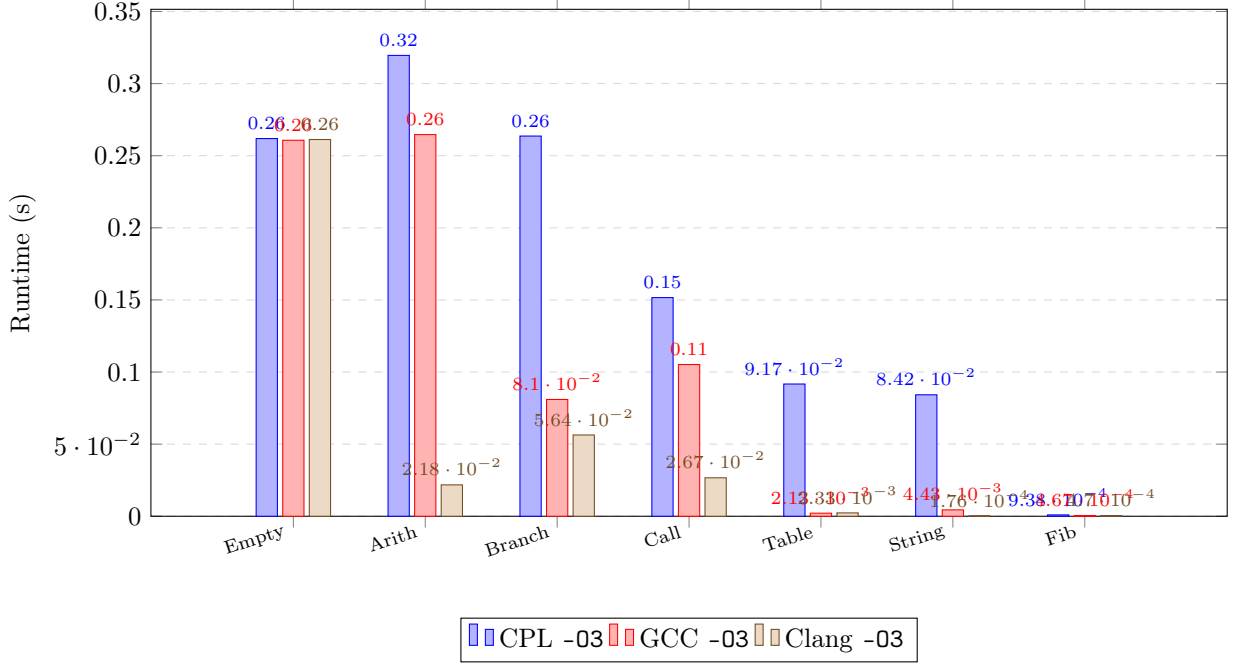
Рис. 3: x86_64 optimized runtimes for the benchmark kernels. The full x86_64/i386 table is reported in Table 9.
