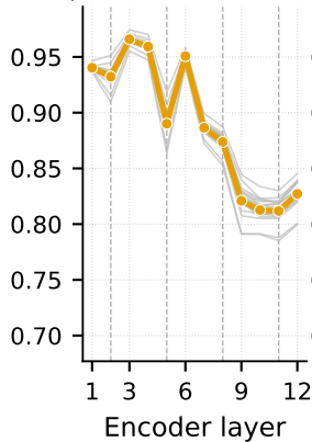
whisper-small (244M, L=12)
