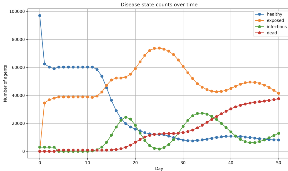
Figure 1: 50 Day simulation for N=100000
