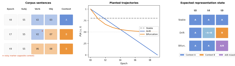
Fig. 1. Benchmark design overview. Left: SVO sentences for a drifting subject across three epochs; a context-A verb appearing in a context-B sentence at t7 (marked *) illustrates the deliberate noise in local markers. Center: planted P(A | s, t) trajectories for Stable (flat), Drift (monotonic), and Bifurcating (levelling at 0.5) subjects across t0 – t9 . Right: expected nearest-neighbor behavior for a traceable representation.
