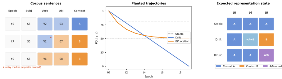
Fig. 1. Benchmark design overview. Left: SVO sentences for a drifting subject across three epochs; an N_1 verb appearing in an N_2 sentence at t7 (marked *) illustrates the deliberate noise in local markers. Center: planted P(N_1 | s, t) trajectories for Stable (flat), Drift (monotonic), and Bifurcating (levelling at 0.5) subjects across t0 – t9 . Right: expected nearest-neighbor behavior for a traceable representation.
