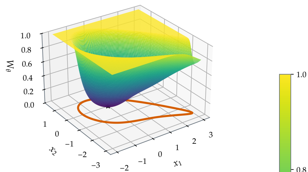
Example VI.1 (Two-machine) Learned Lyapunov function
