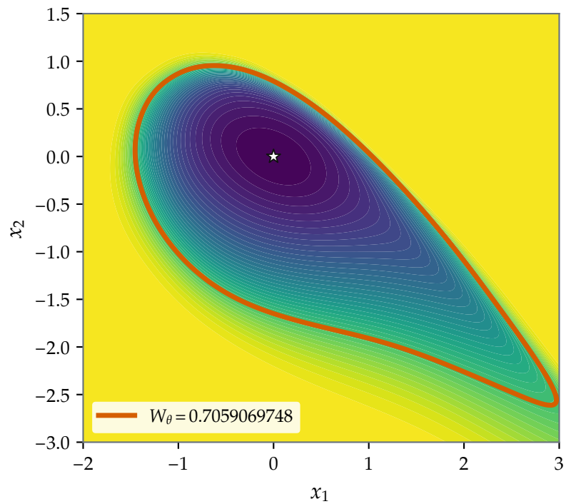
Example VI.1 (Two-machine) Verified level set
