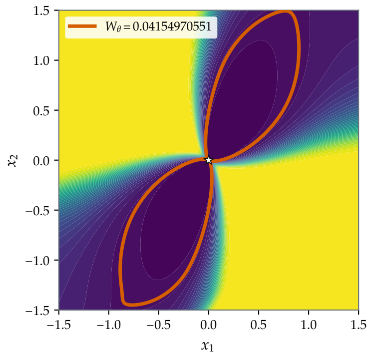
Example VI.2 (Cubic core) Verified level set
