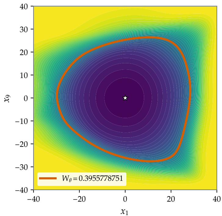
Example VI.3 (10D) Tested level set
