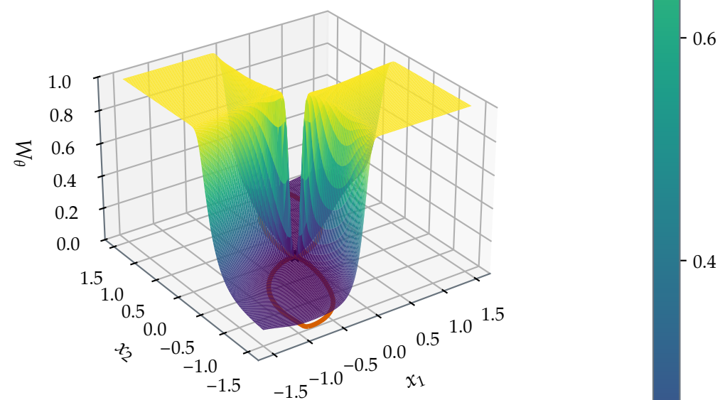
Example VI.2 (Cubic core) Learned Lyapunov function
