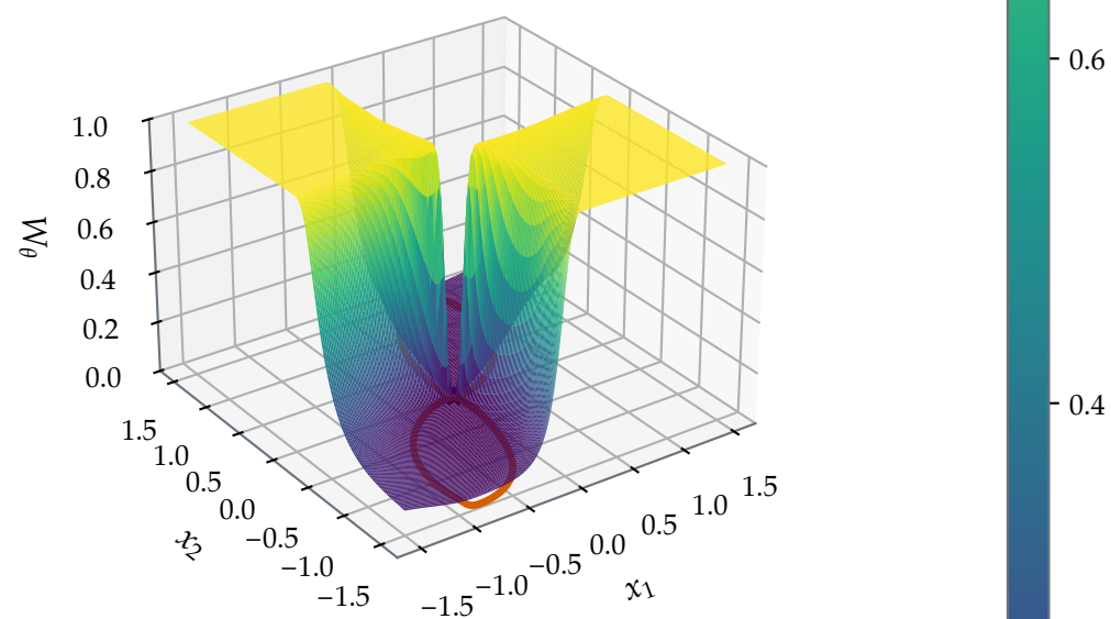
Example VI.2 (Cubic core) Learned Lyapunov function
