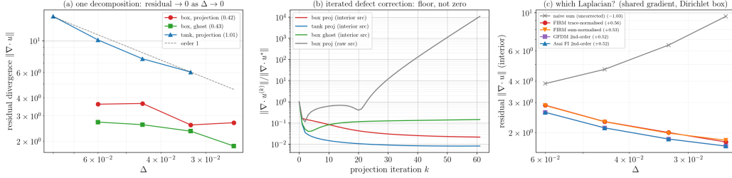
Helmholtz–Hodge decomposition with the renormalised FIRM operators
