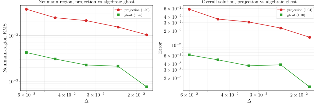
Wedge tank, seed-averaged convergence
