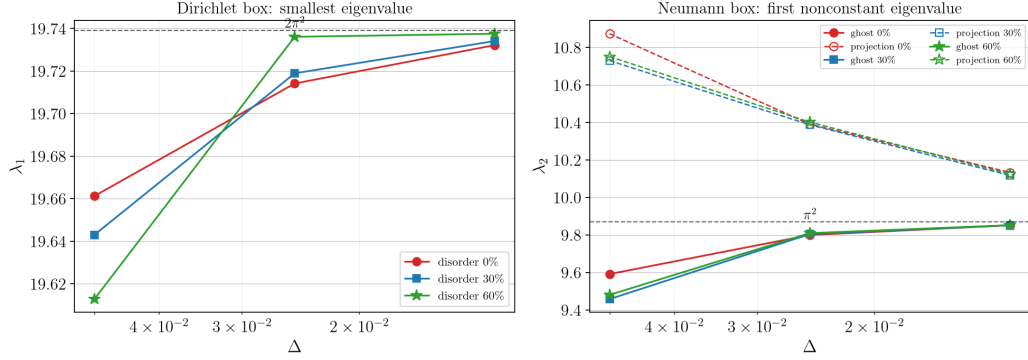
Figure 19: Smallest eigenvalues of the row-scaled closed operator against the spacing \Delta . The Dirichlet square converges to the continuous 2\pi^2 at every disorder level, and the first nonconstant eigenvalue of the all-Neumann box converges to \pi^2 under the ghost closure.
