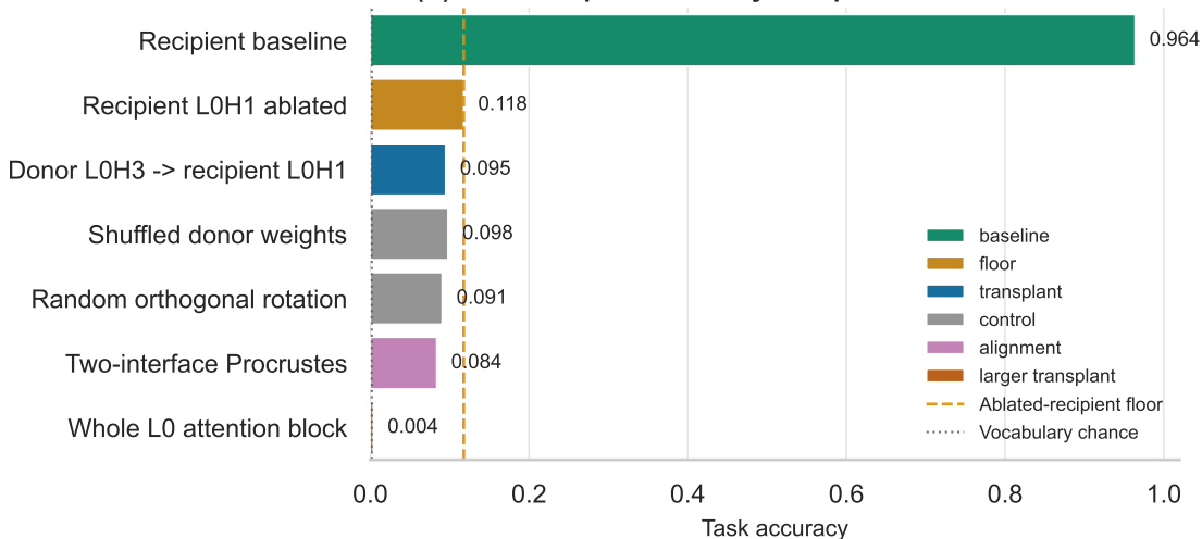
(B) Raw transplant accuracy collapses to the ablated floor
