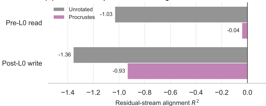
(C) Procrustes improves residual alignment but remains below zero
