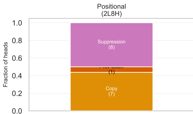
Figure 2: Head Role Distributions Across Three Tasks
