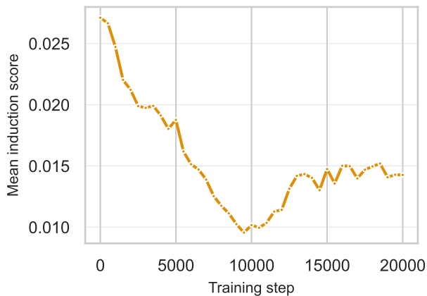
Mean QK Induction Score (full training)
