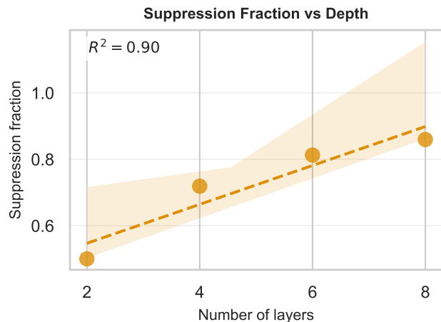
Figure 4: Depth Scaling of Suppression Cascade
