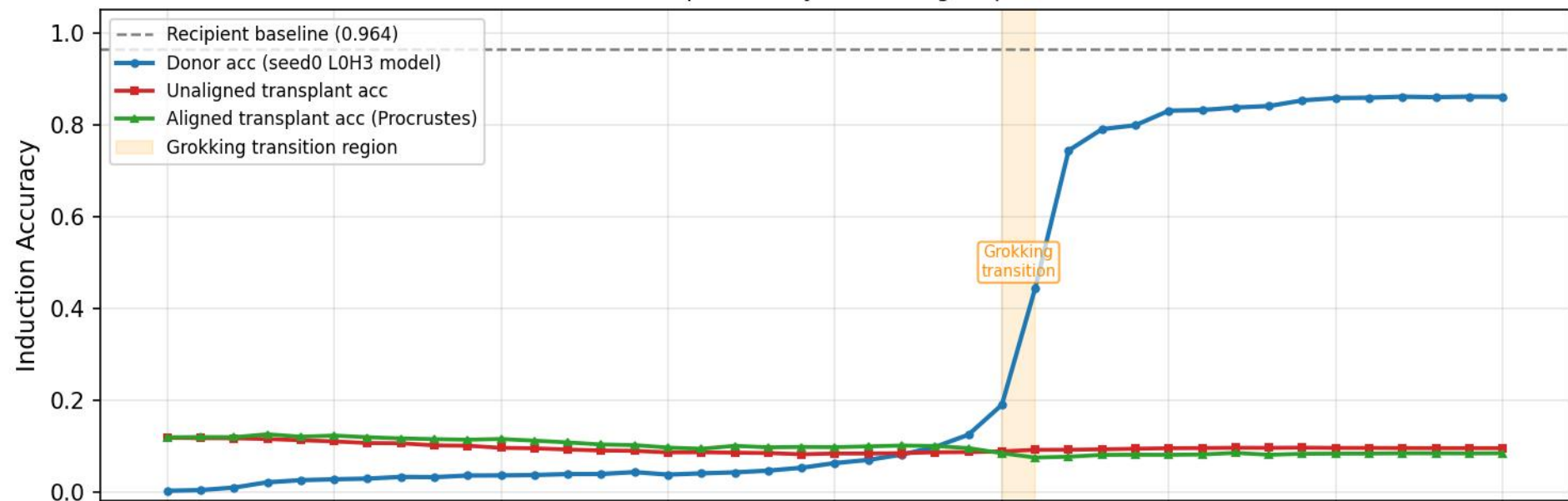
Top: Accuracy vs. Training Step
