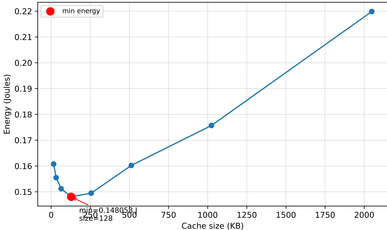
L1 data cache (C1)
