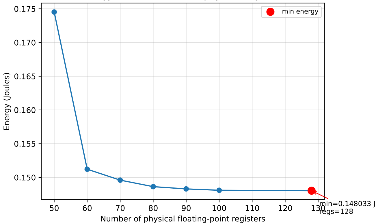
Energy vs number of float physical registers
