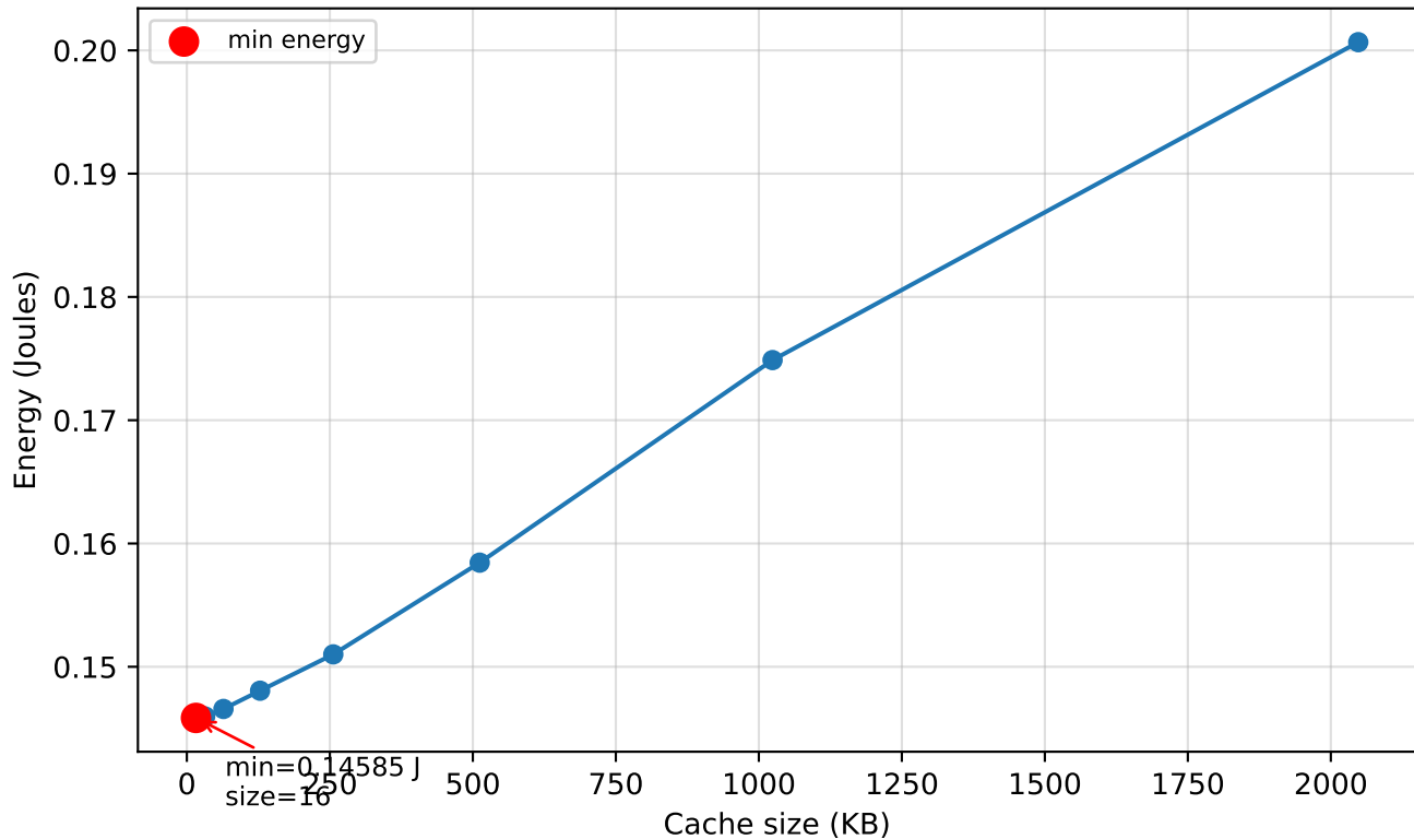
L1 instruction cache (INSTR)
