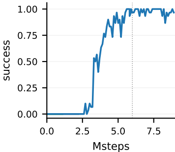
peg-insert-side
