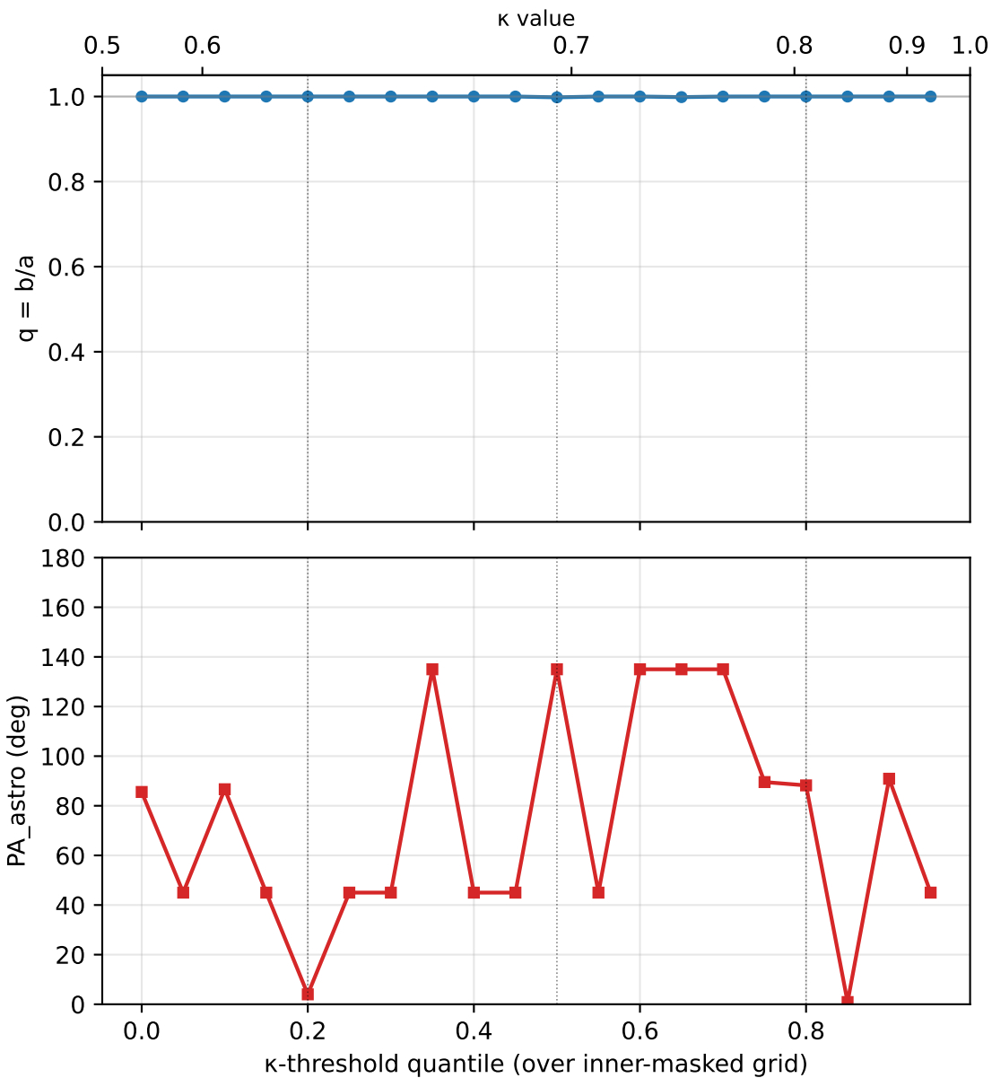
ARCH ellipticity vs \kappa threshold (NFW)
