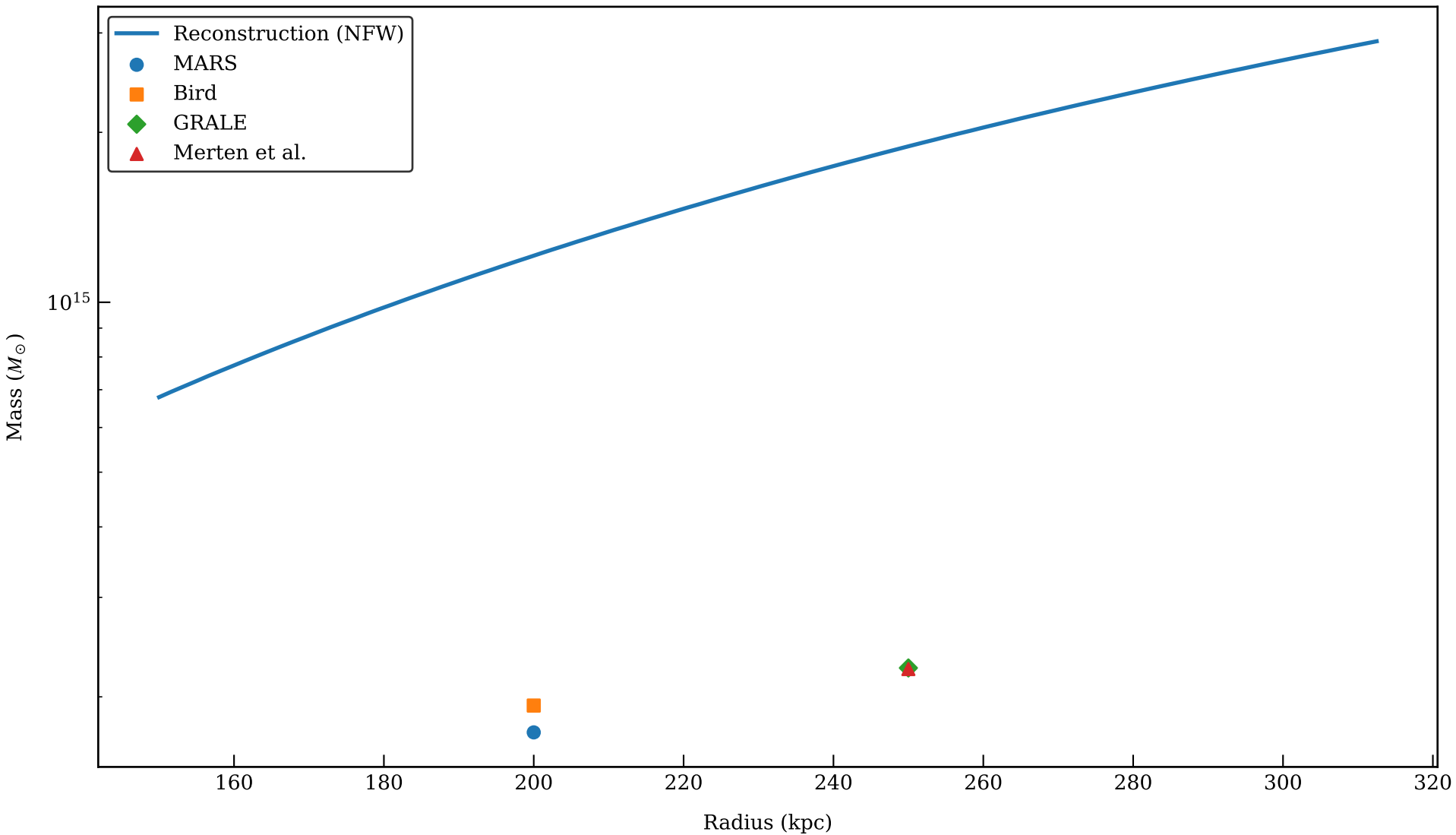
Mass Comparison: ABELL_2744 (NFW, WL+SL (two-pass), signals: f_g)
