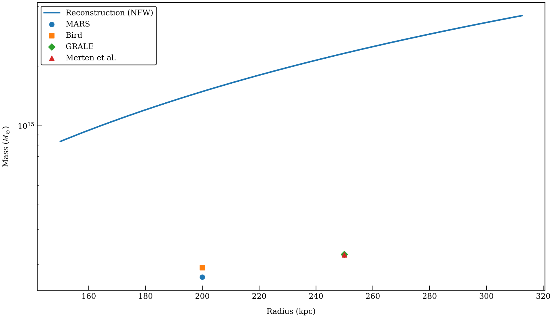
Mass Comparison: ABELL_2744 (NFW, WL+SL (two-pass), signals: shear_g)
