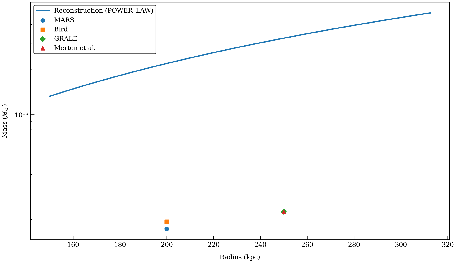
Mass Comparison: ABELL_2744 (POWER_LAW, WL+SL (two-pass), signals: f_g)
