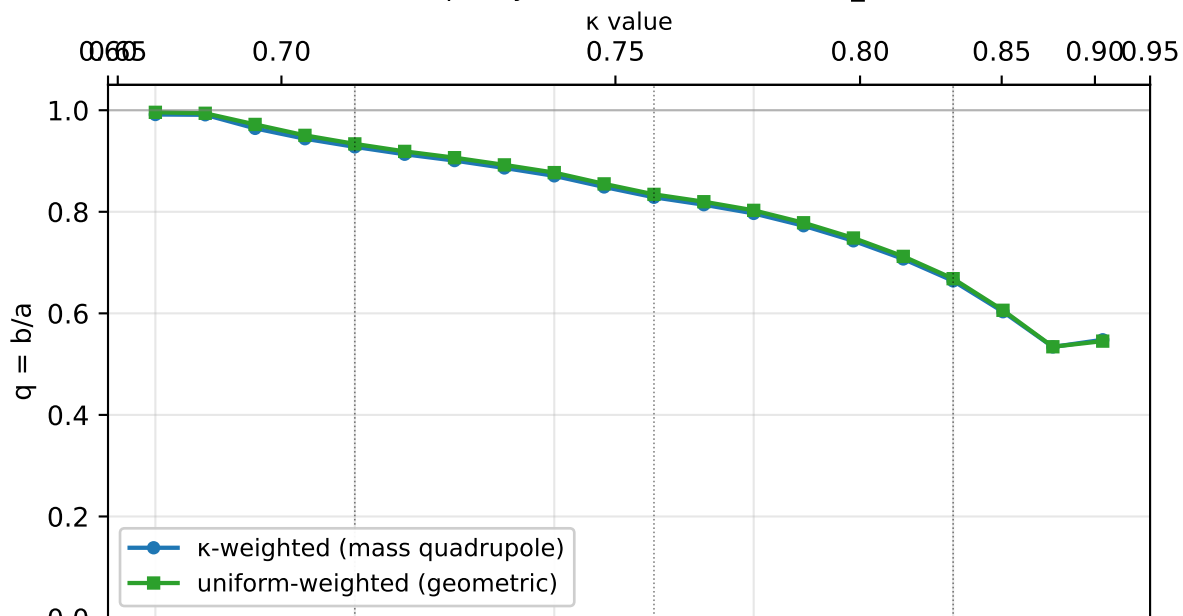
ARCH ellipticity vs \kappa threshold (POWER_LAW)
