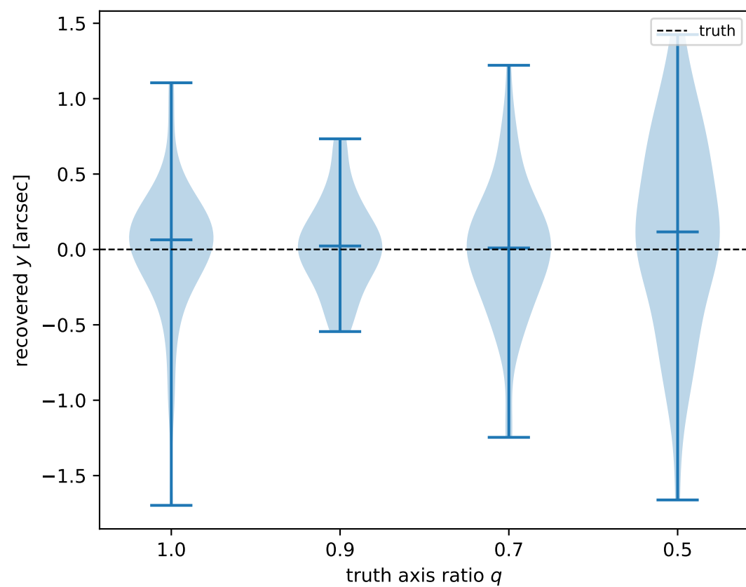
Parameter recovery under circularity: elliptical power-law truth
