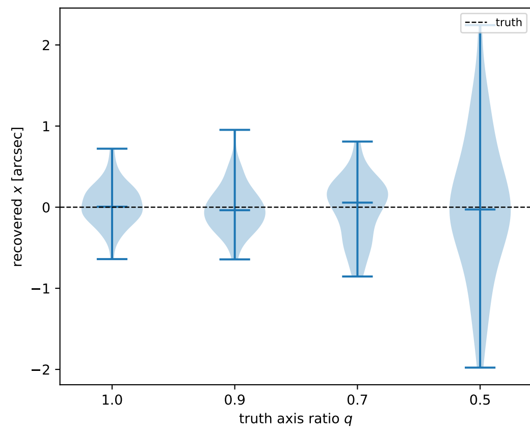
Parameter recovery under circularity: elliptical power-law truth
