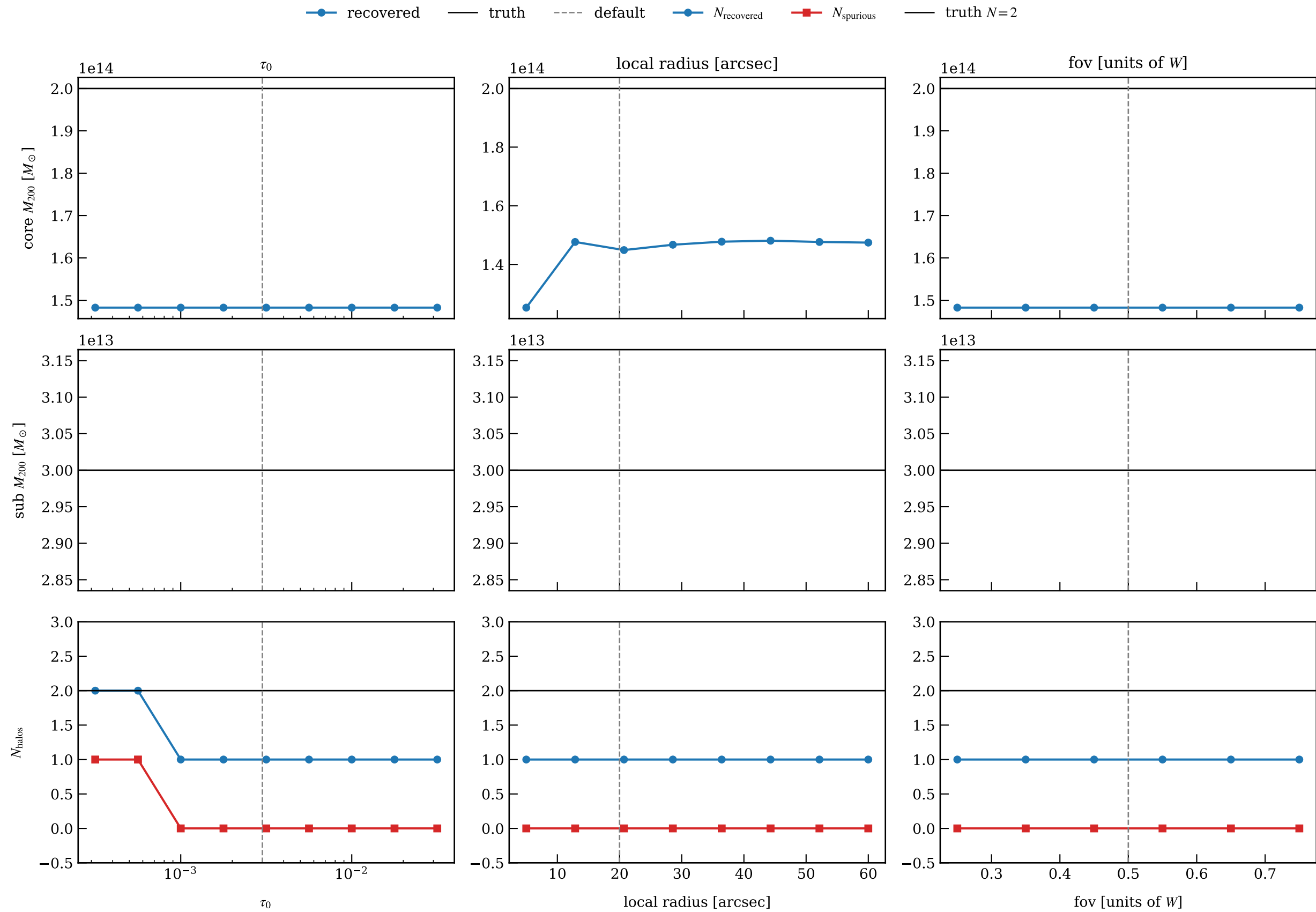
Hyperparameter sensitivity (n_seeds = 1, n_sources = 500, injected: core 2.0e+14 + sub 3.0e+13 M_\odot )
