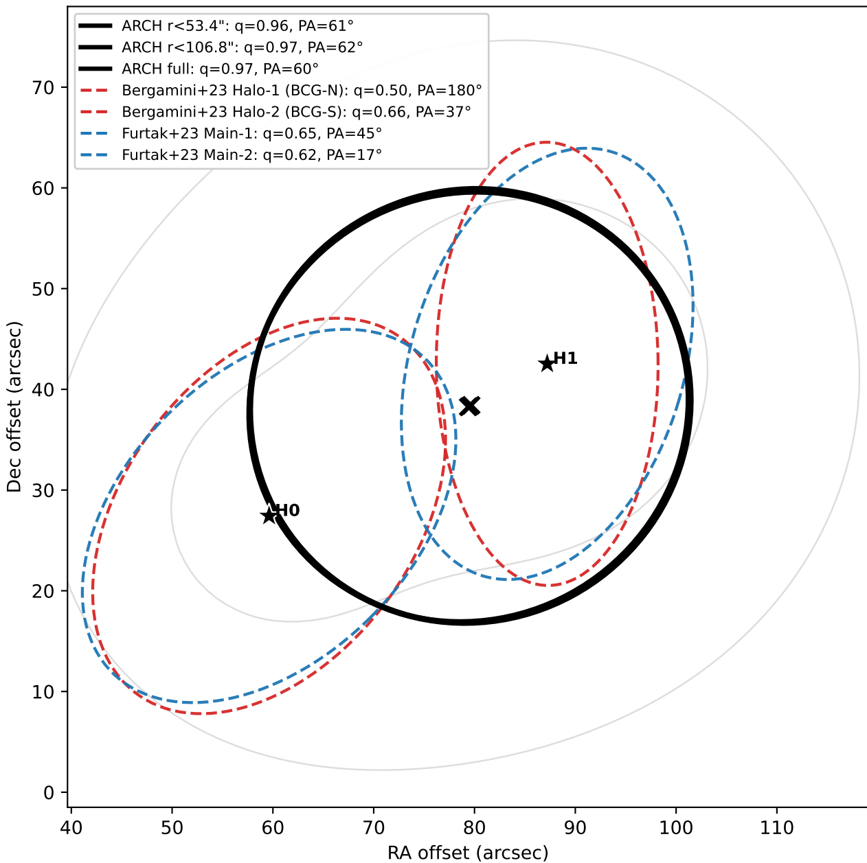
\kappa ellipticity — ARCH vs literature (ARCH sheet subtracted q=0.20 )
