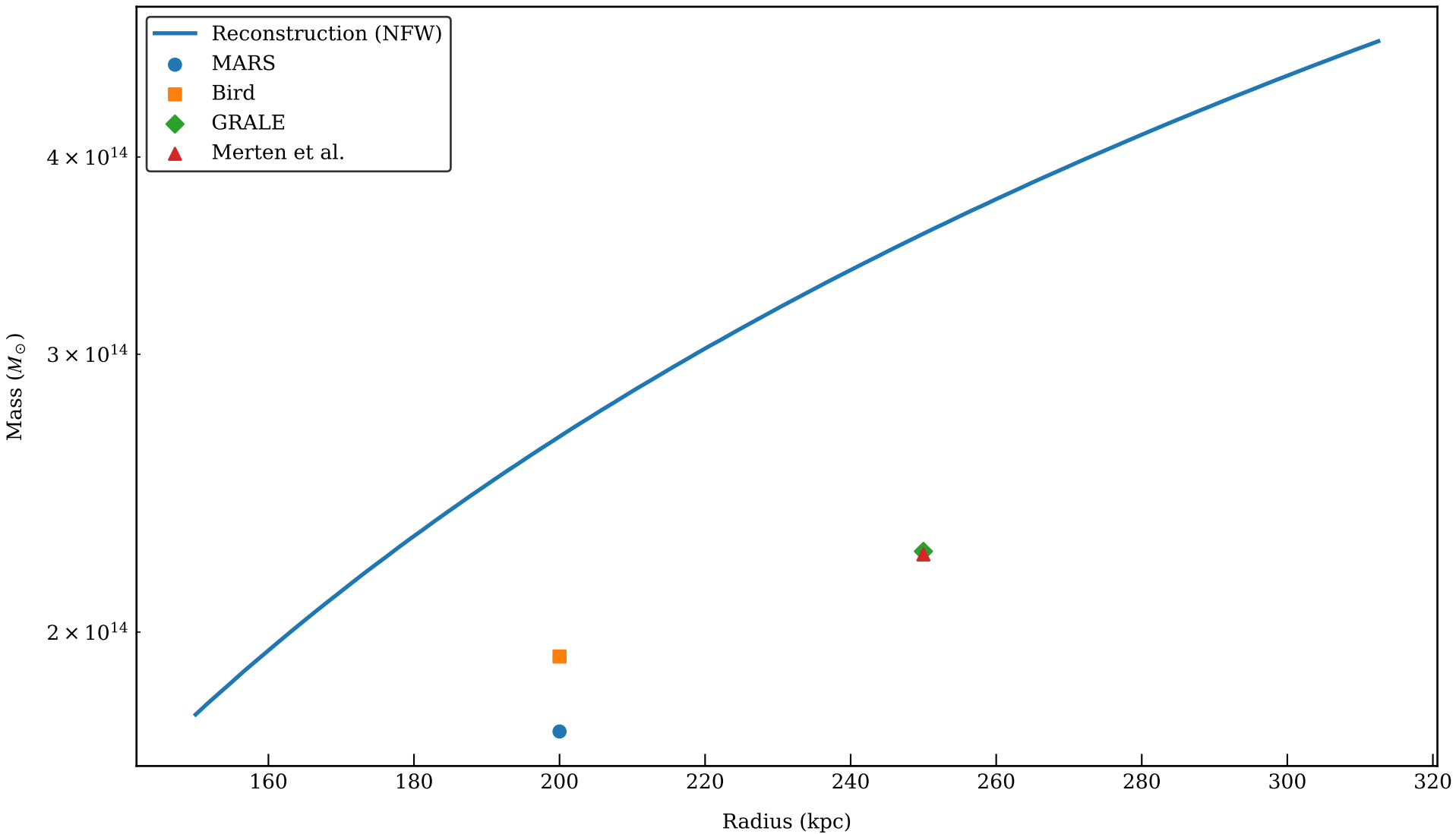
Mass Comparison: ABELL_2744 (NFW, signals: shear_f)
