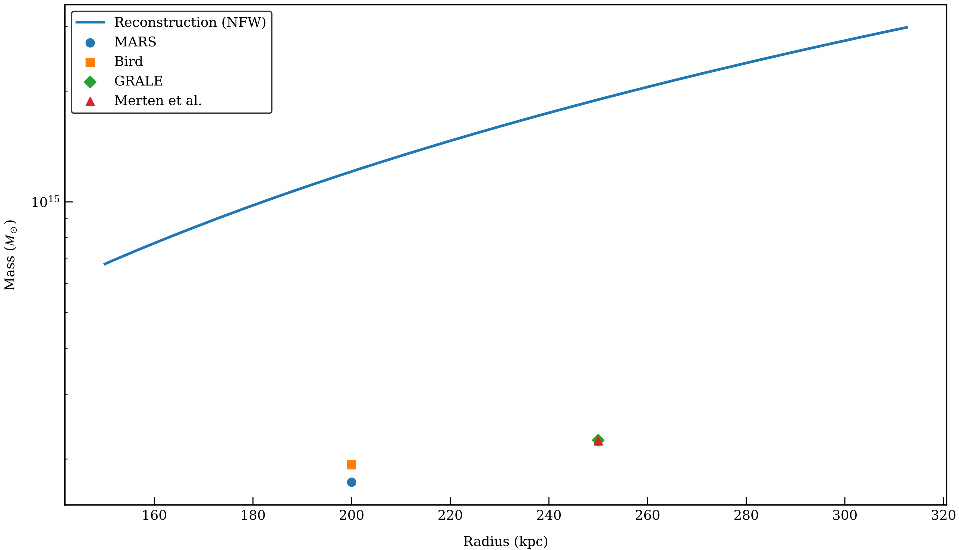
Mass Comparison: ABELL_2744 (NFW, WL+SL, signals: shear_f)
