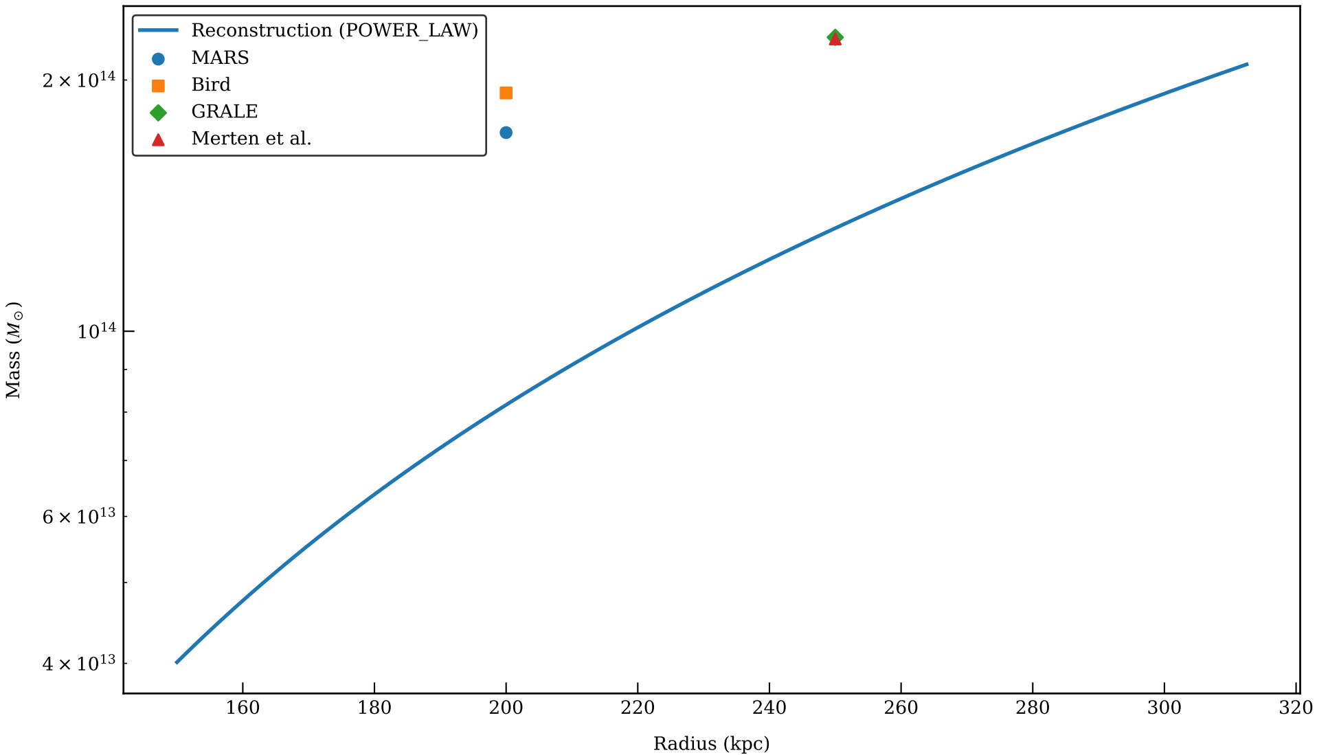
Mass Comparison: ABELL_2744 (POWER_LAW, WL+SL, signals: all)
