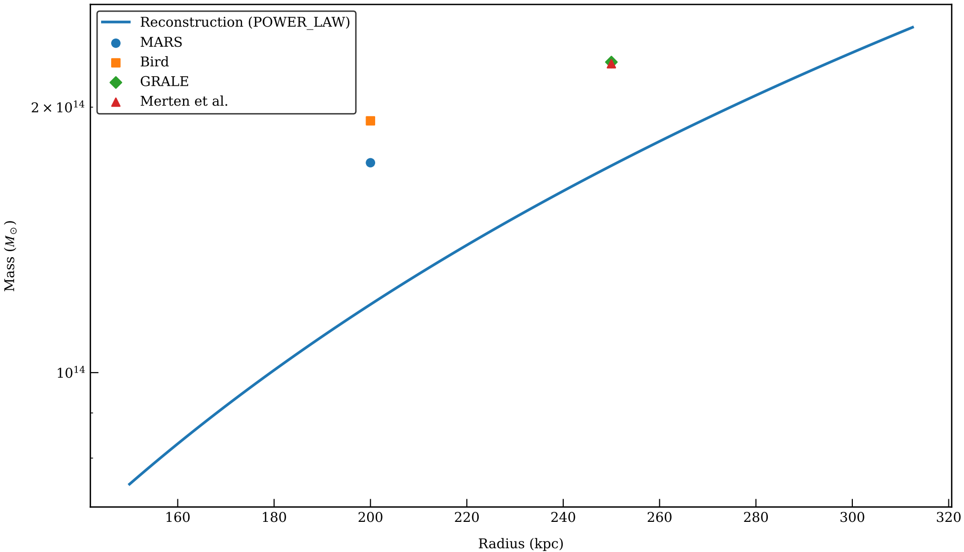
Mass Comparison: ABELL_2744 (POWER_LAW, WL+SL, signals: shear_g)
