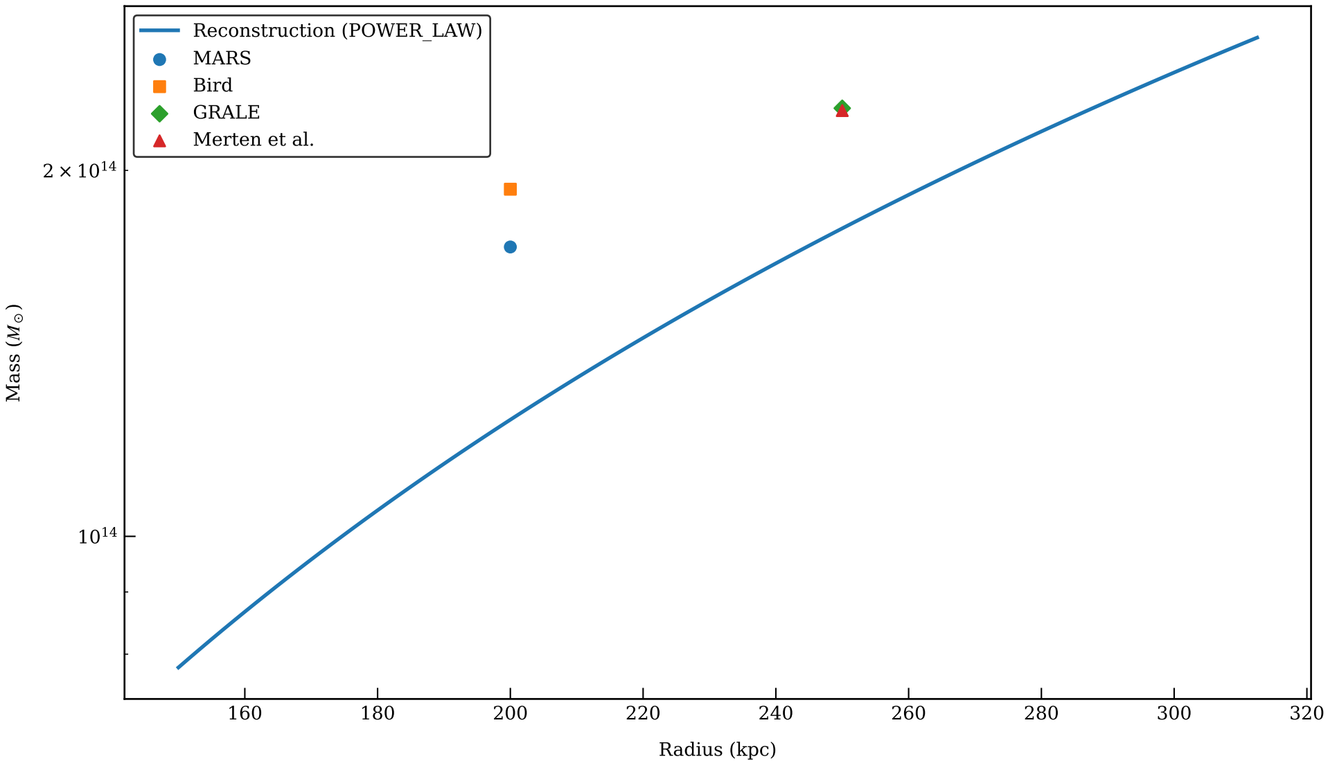
Mass Comparison: ABELL_2744 (POWER_LAW, WL+SL (two-pass), signals: shear_g)
