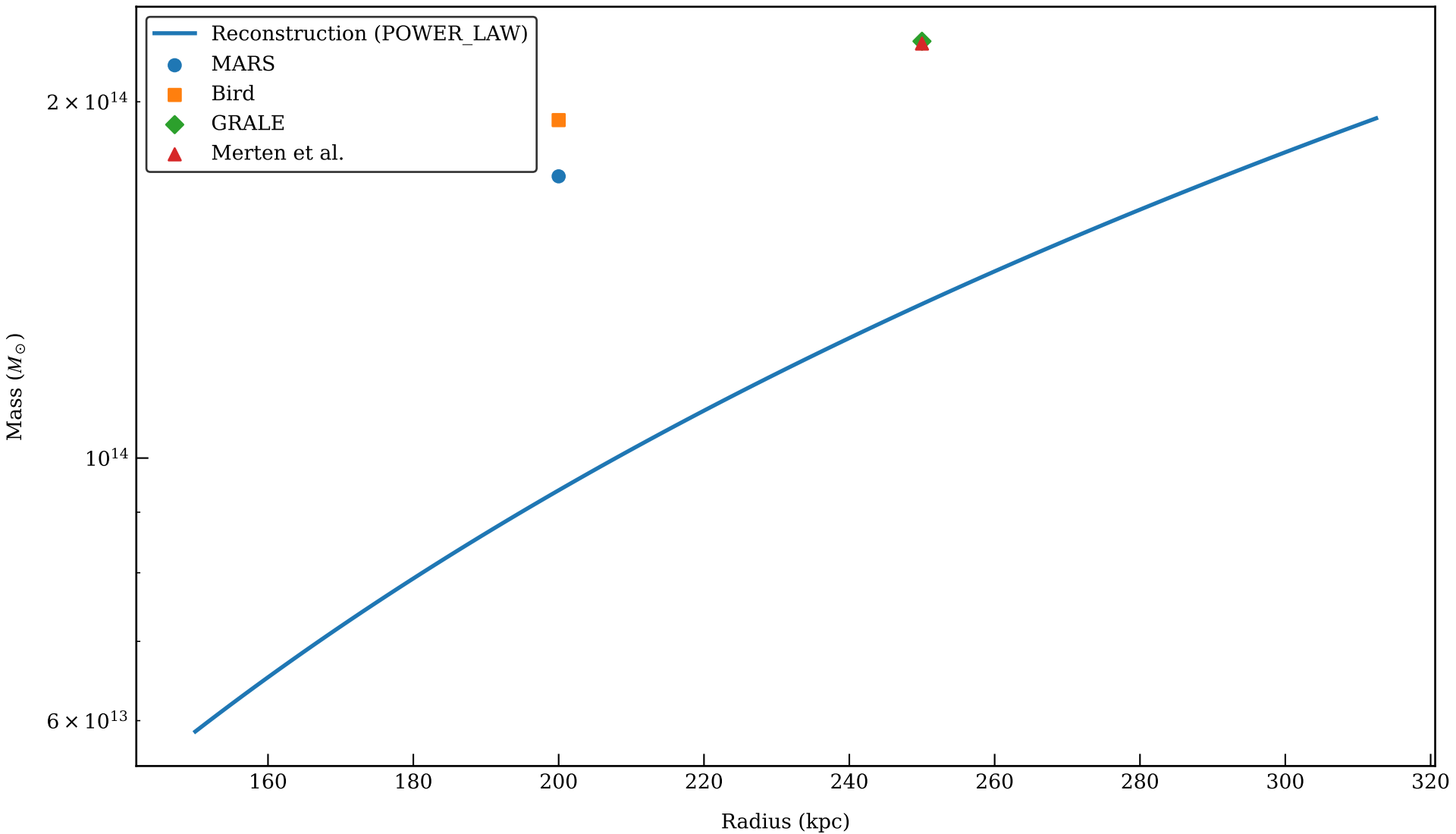
Mass Comparison: ABELL_2744 (POWER_LAW, signals: all)
