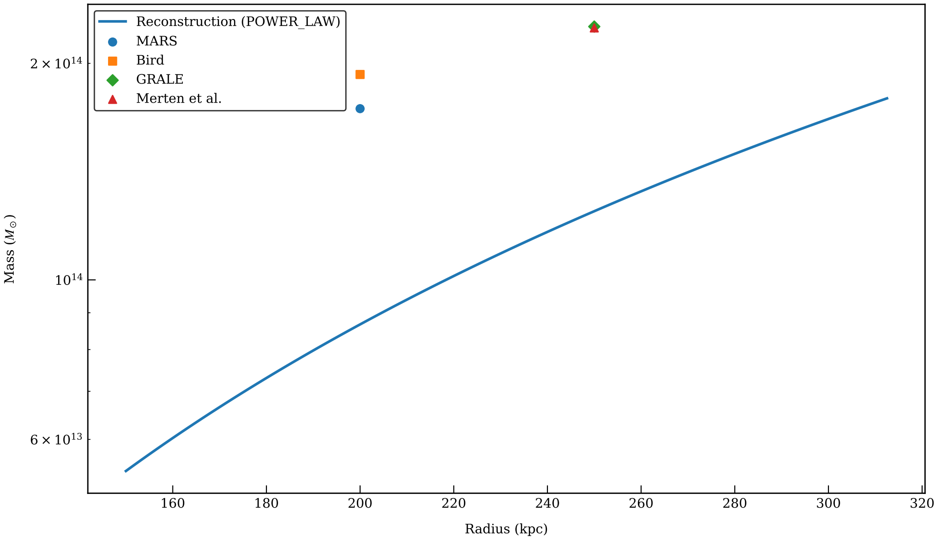
Mass Comparison: ABELL_2744 (POWER_LAW, signals: all)
