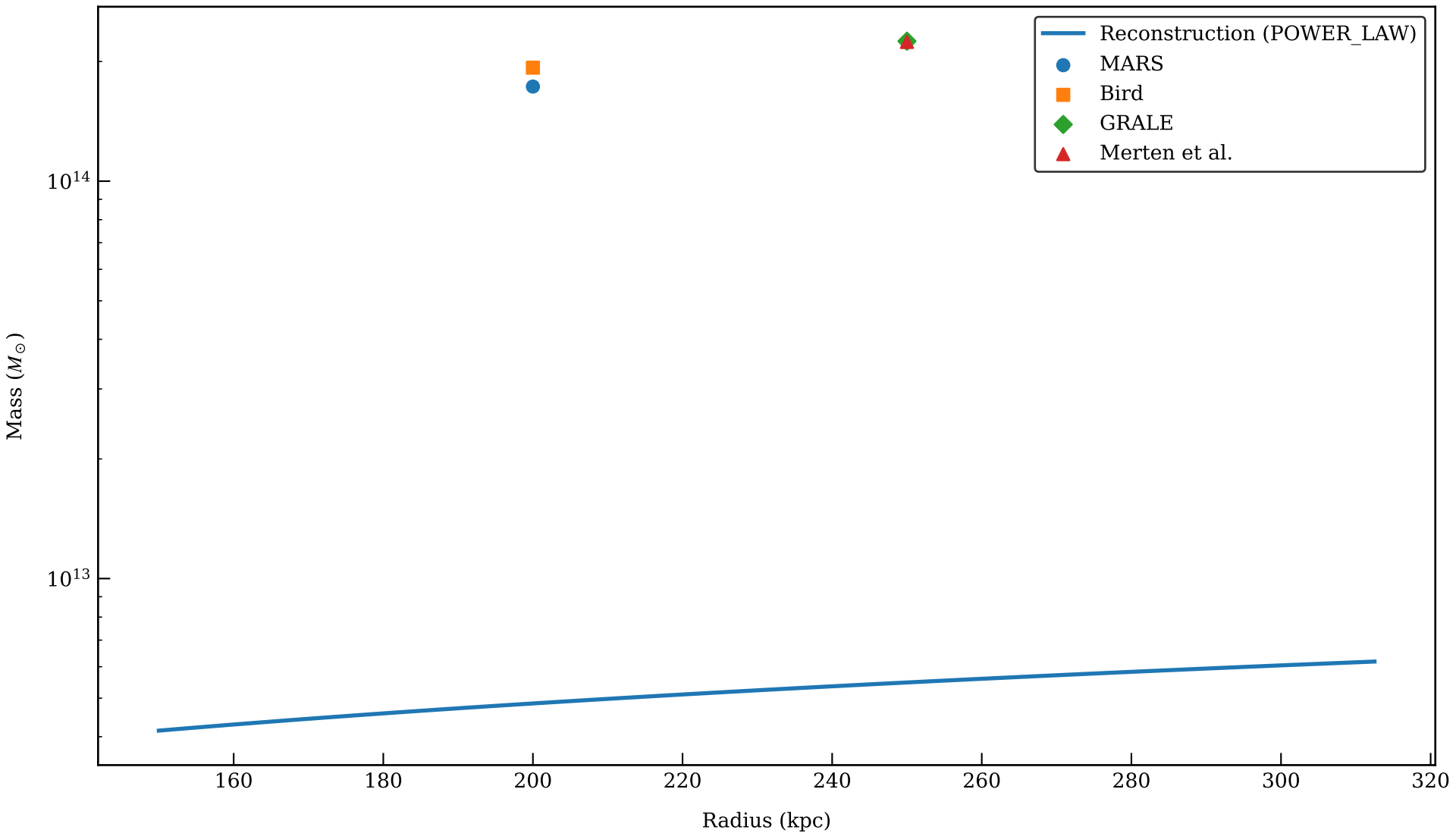
Mass Comparison: ABELL_2744 (POWER_LAW, signals: f_g)
