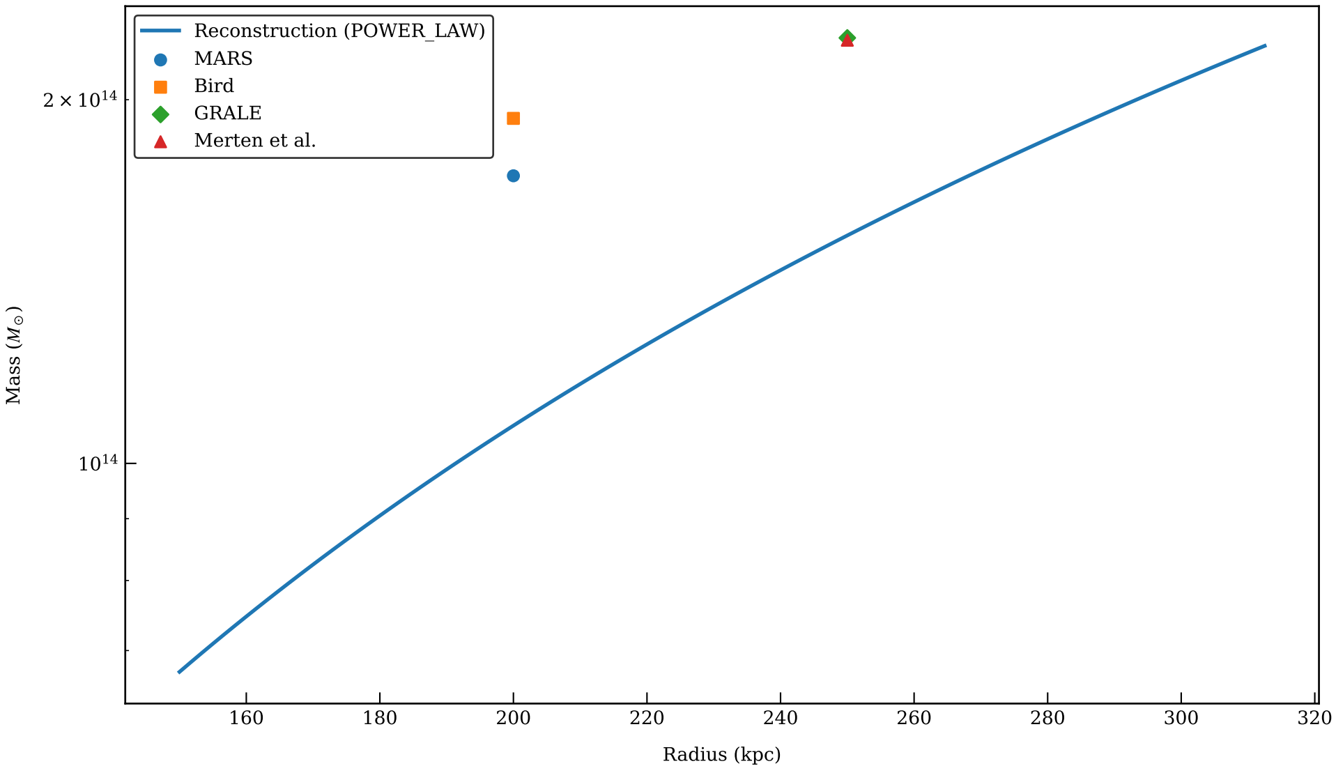
Mass Comparison: ABELL_2744 (POWER_LAW, signals: shear_f)
