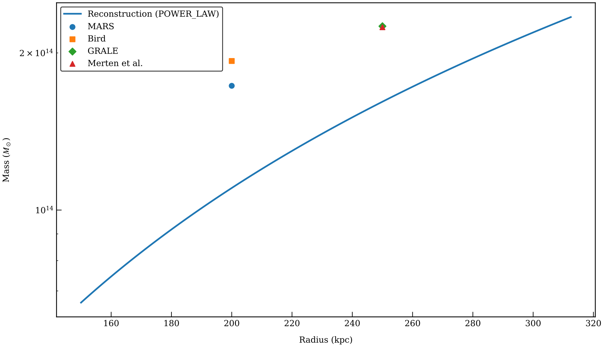
Mass Comparison: ABELL_2744 (POWER_LAW, signals: shear_g)
