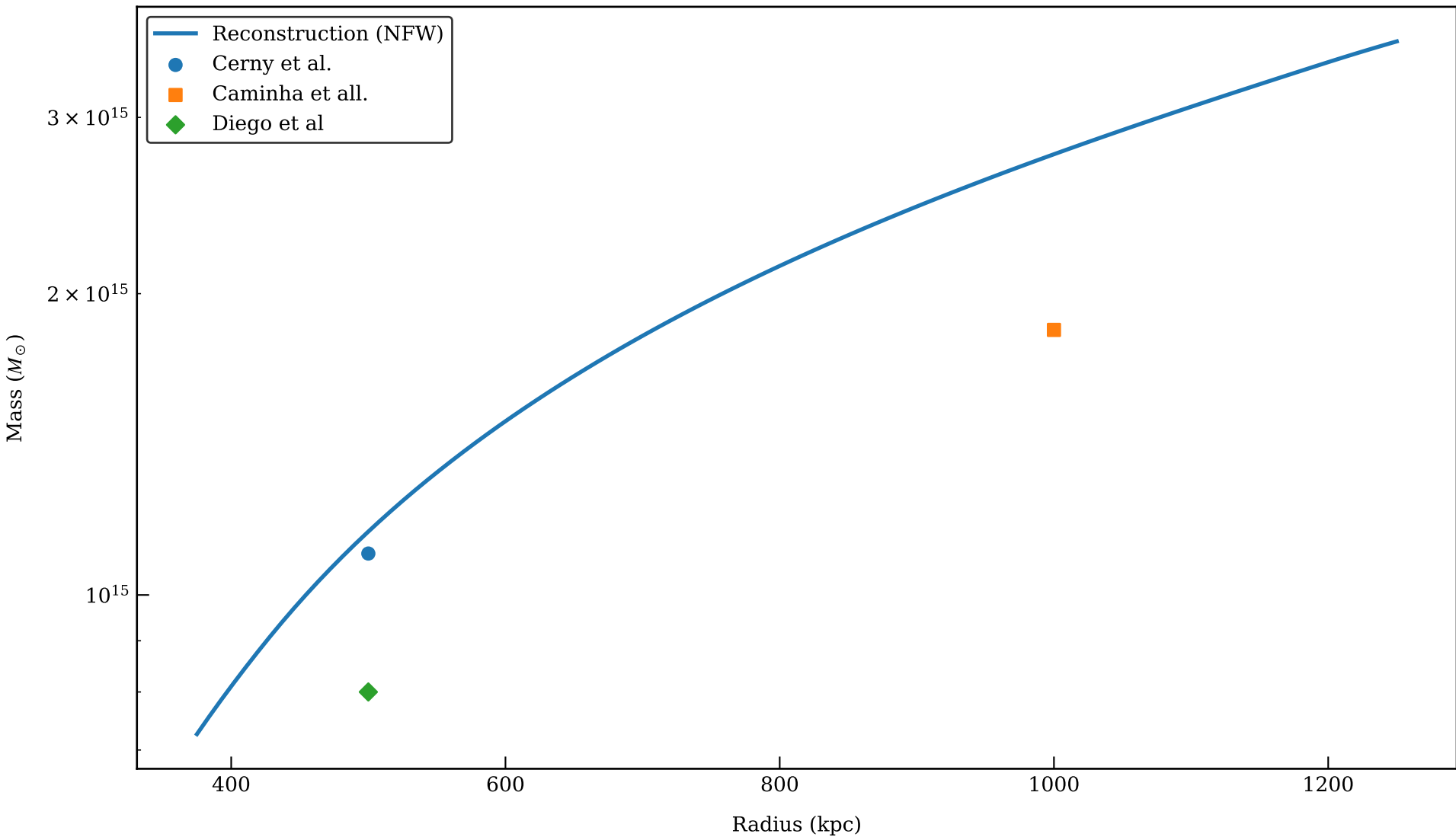
Mass Comparison: EL_GORDO (NFW, signals: all)
