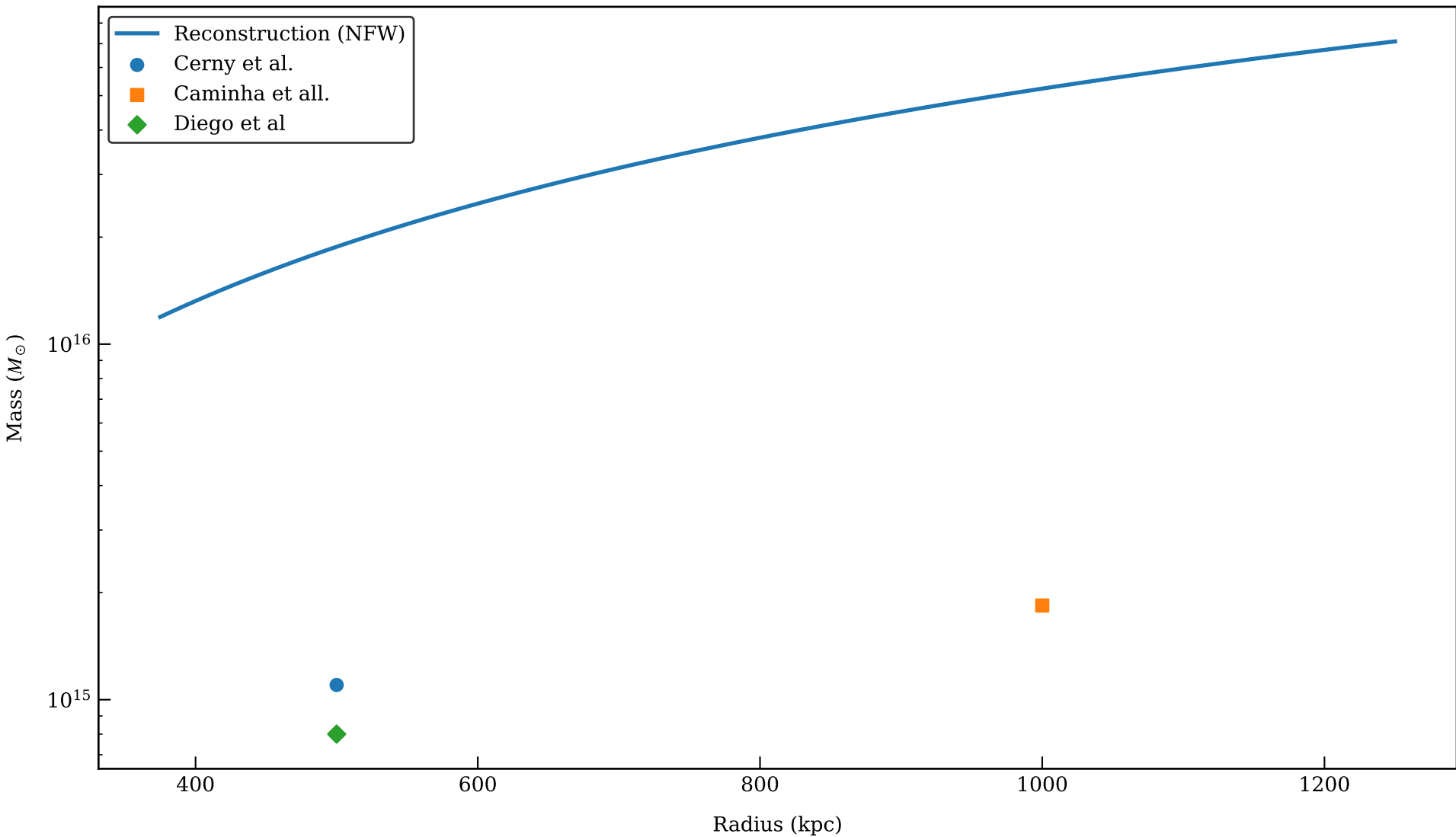
Mass Comparison: EL_GORDO (NFW, signals: f_g)
