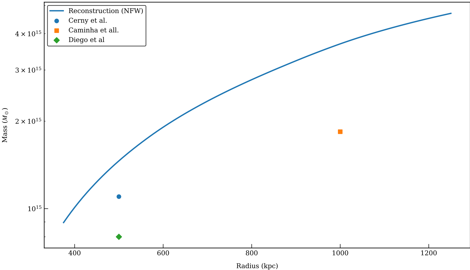
Mass Comparison: EL_GORDO (NFW, signals: shear_f)
