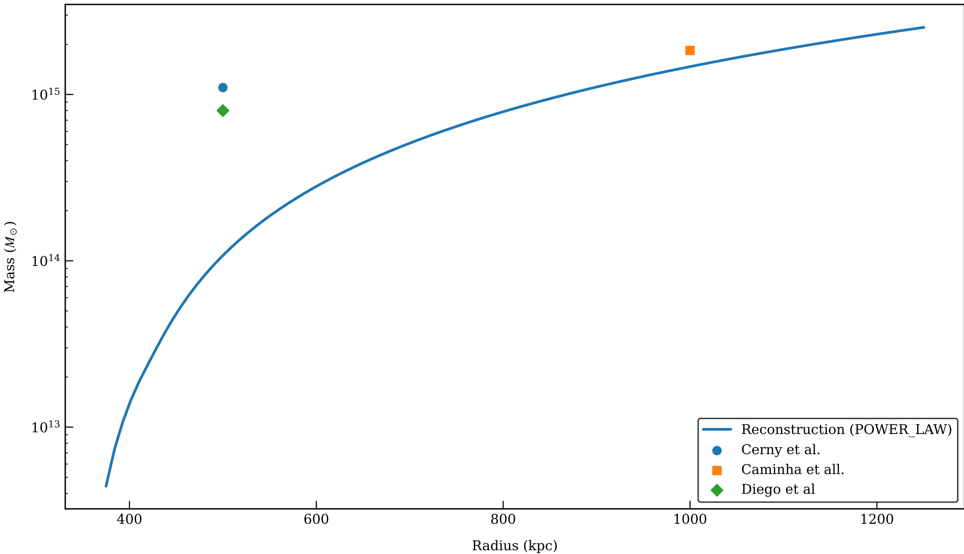
Mass Comparison: EL_GORDO (POWER_LAW, signals: shear_f)
